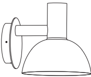
Measurements H: 20 cm, D: 26 cm Shade Ø: 20 cm Base mount Ø: 10,5 cm
